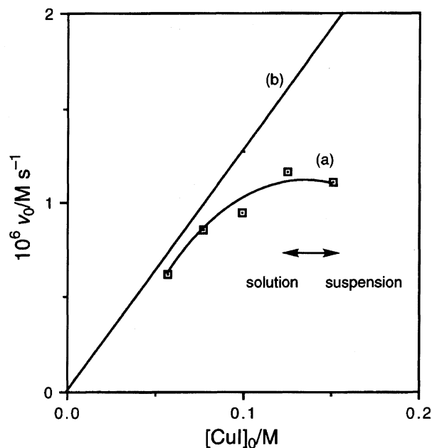
Fig. 3. (a) Kinetic plot under the conditions of near saturation of CuI. [2d]_0 = 2.5 \times 10^{-2} M, in acetonitrile at 40^\circ\text{C} . (b) Theoretical plot according to Eq. 3.
