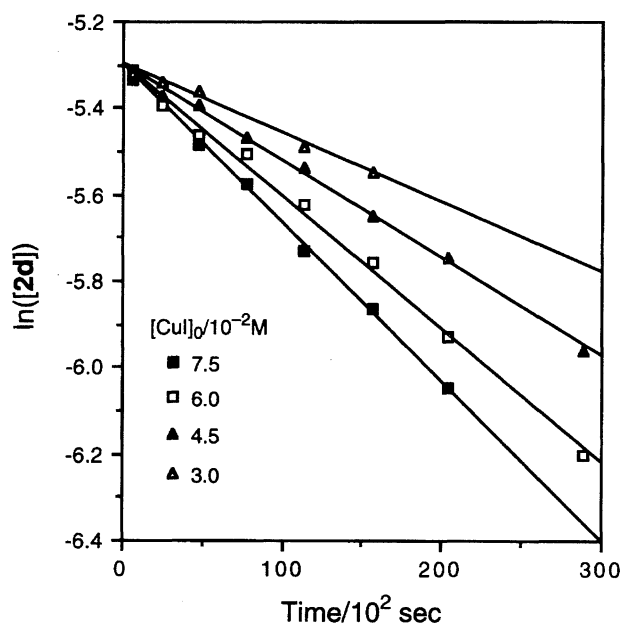
Fig. 2. Kinetic dependence on CuI concentration. [2d]_0 = 5.0 \times 10^{-3} M in acetonitrile at 40^\circ\text{C} .
