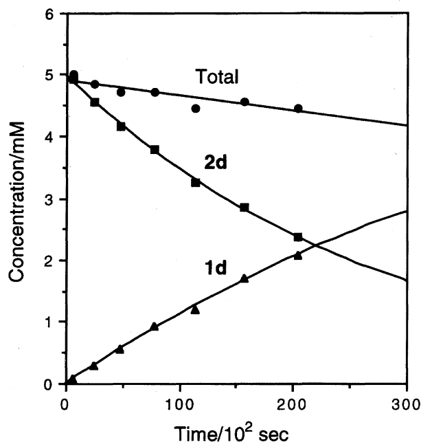
Fig. 1. Reaction profile for the iodination of 2d ( 5.0 \times 10^{-3} M) with CuI ( 7.5 \times 10^{-2} M) in acetonitrile at 40^\circ\text{C} .
